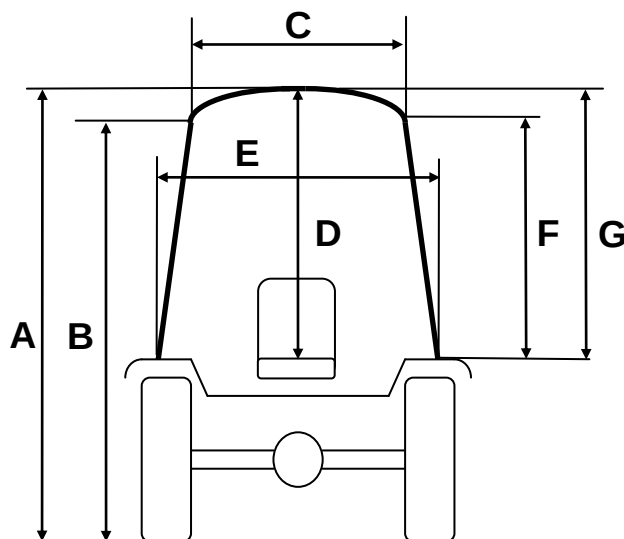
Cabin "COMPACT" NEW HOLLAND T3.80F Back Tyres 360/70 R.24
